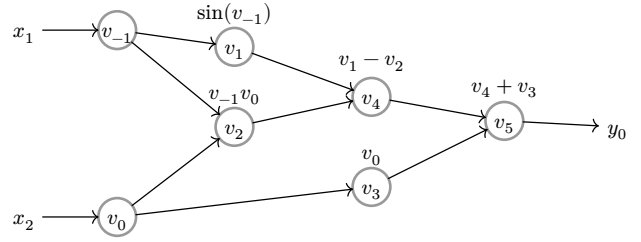
Fig. 1. Computational graph for simple example function.
