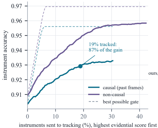
(a) Evidence concentrates the gain
