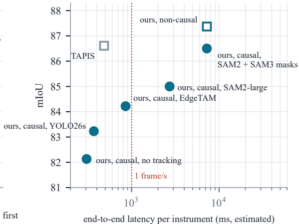
(b) Accuracy against latency
