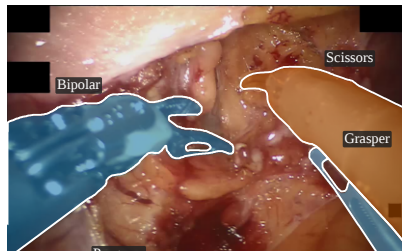
Ground truth
