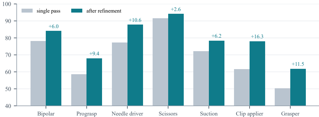
class IoU
