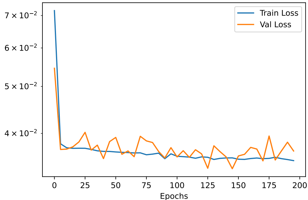
Training and Validation Loss (ConvLSTM)
