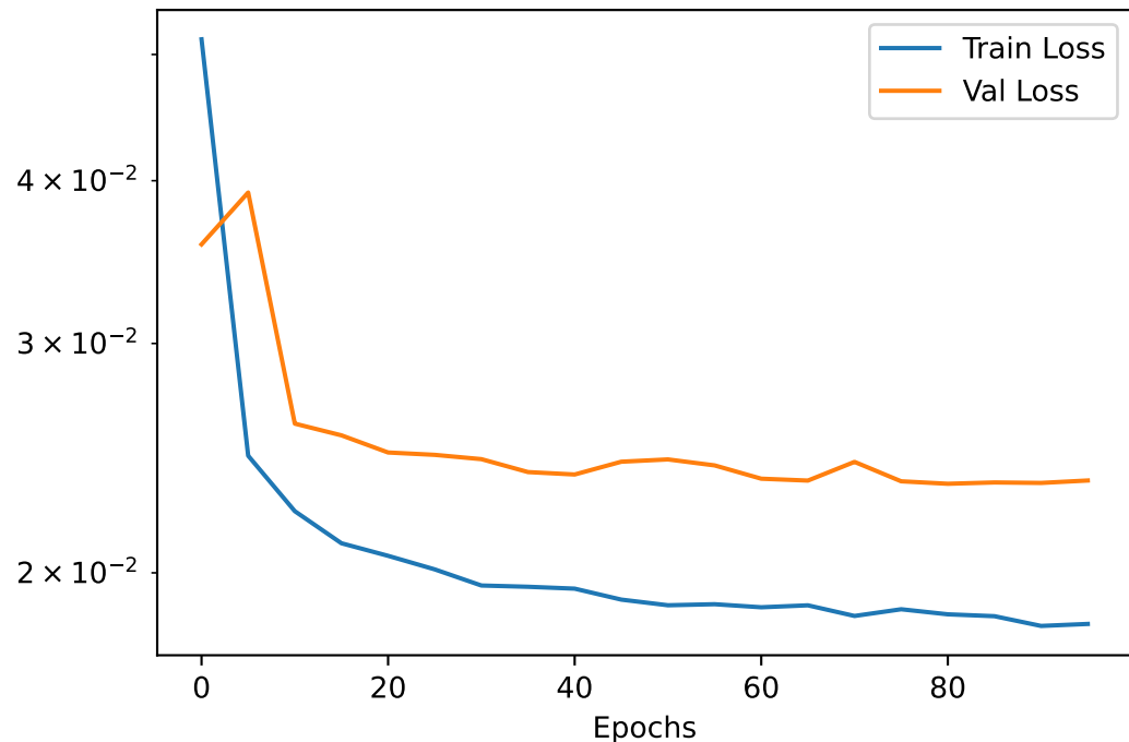
Training and Validation Loss (ConvLSTM (vel.))
