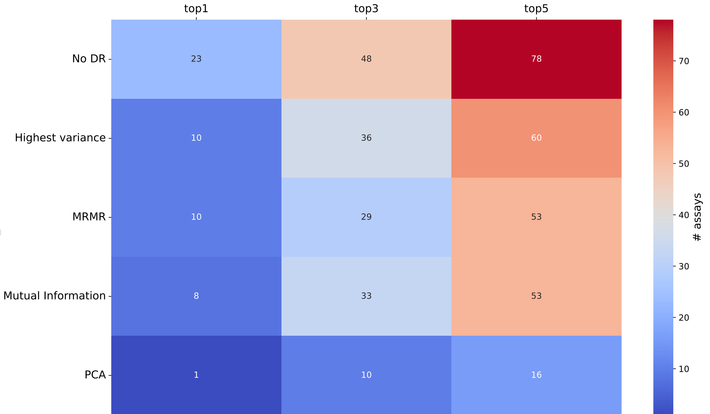
Top-k assay wins per dr_method
