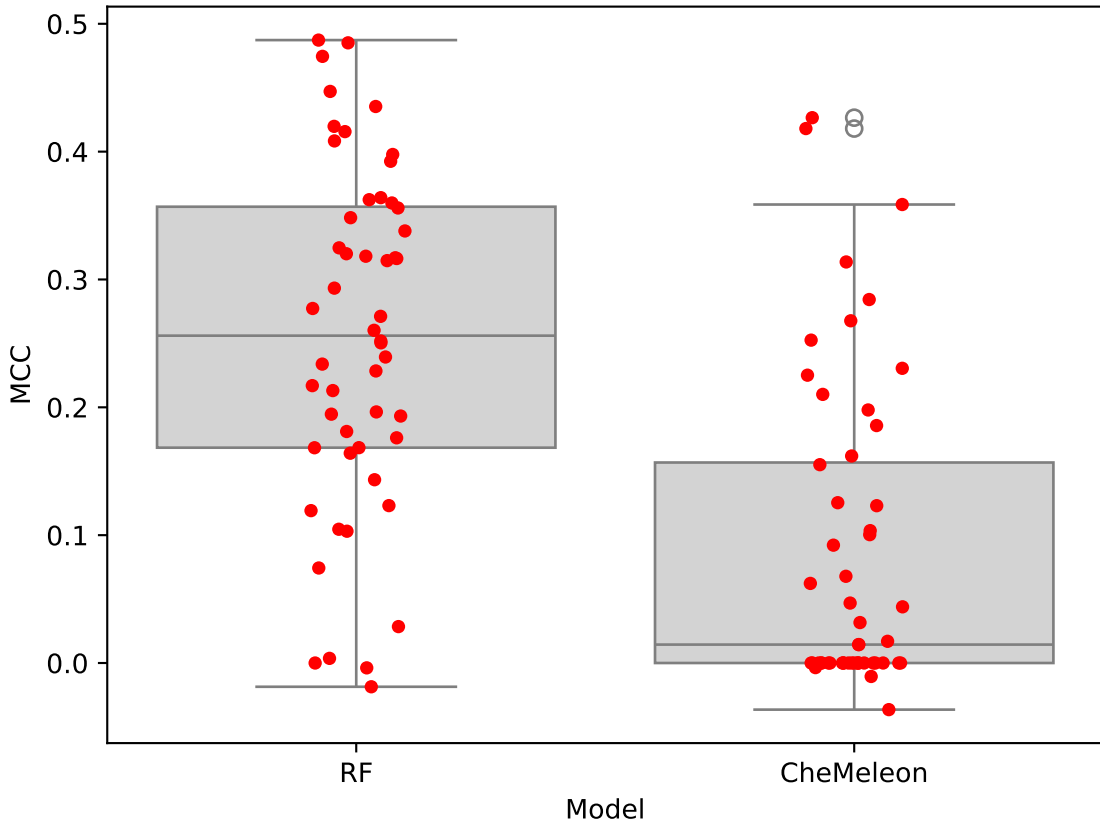
Assay-level Fisher-averaged MCC Wilcoxon p=6.93e-10
