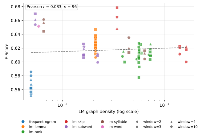
(e) Sentiment—F-measure
