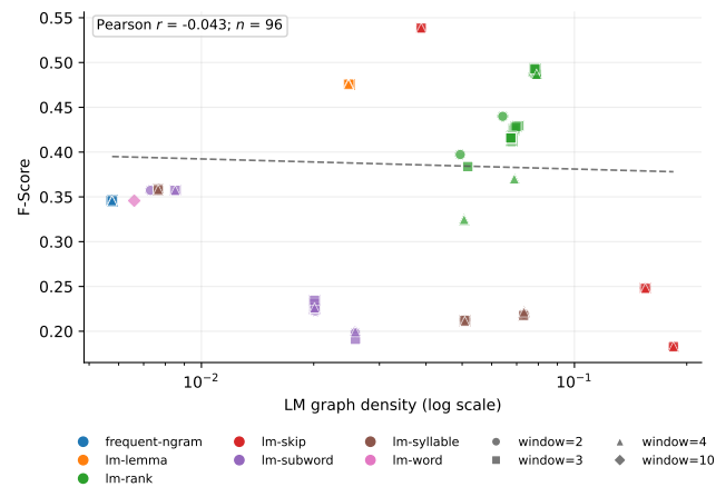
(b) Morphology—F-measure
