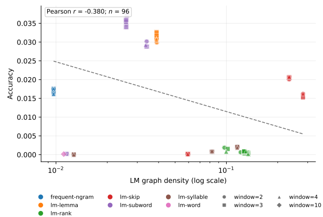
(a) Analogy—Accuracy
