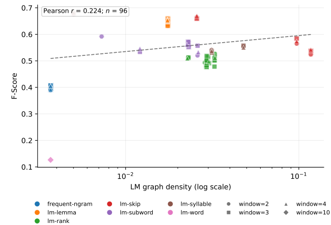
(c) NER—F-measure
