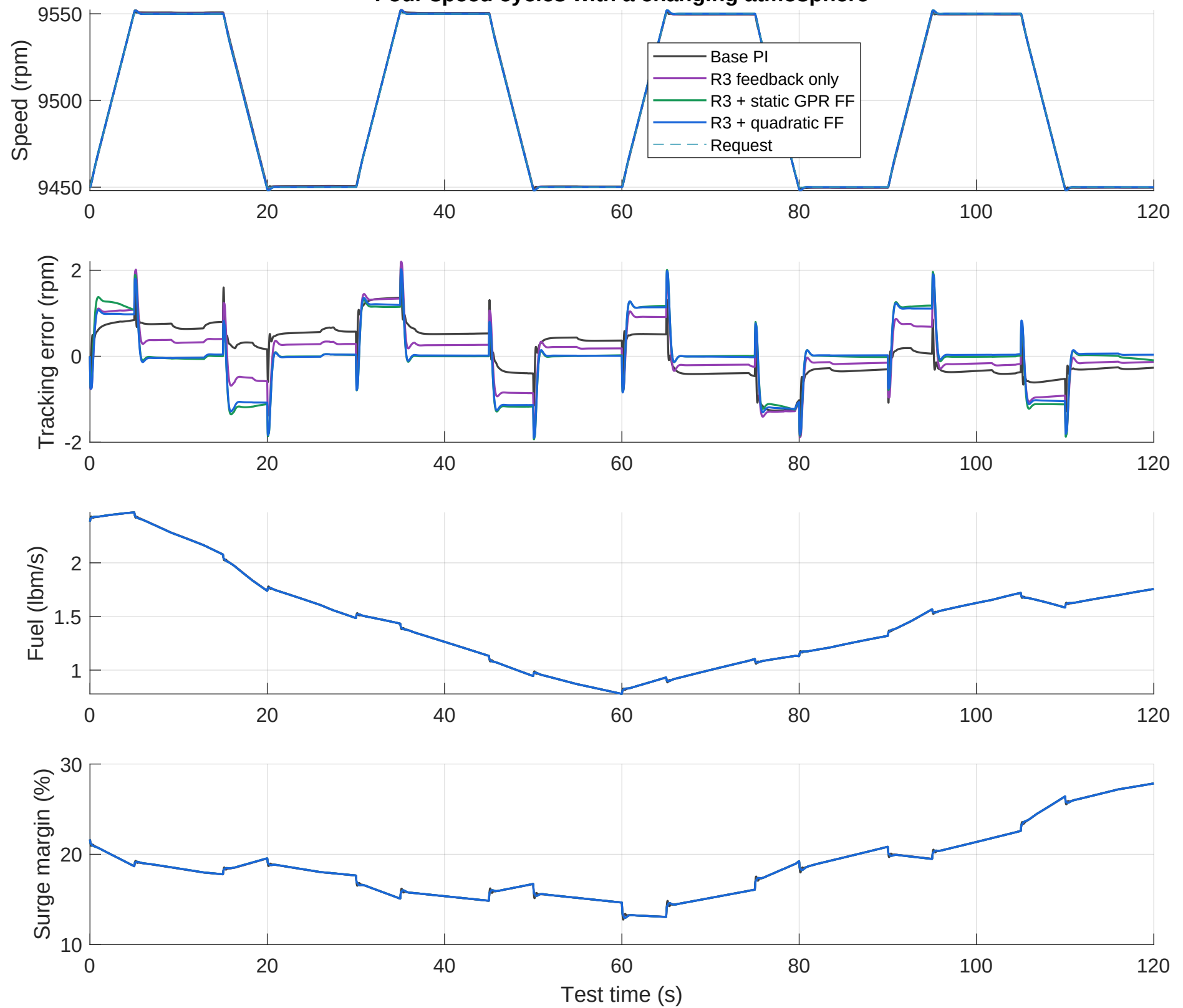
Four speed cycles with a changing atmosphere
