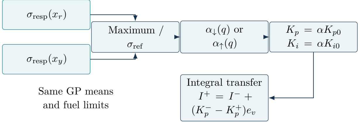
Figure 5.1: Uncertainty-to-gain calculation and integral compensation. The response-SD maximum is a design signal, not a certified loaded-plant error bound.
