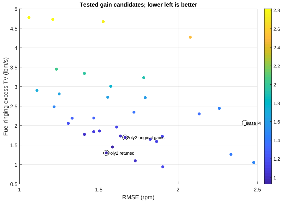
Figure 12.1: All accepted Poly2 gain candidates at 9250 rpm, colored by the joint objective. The best RMSE-only point is not the joint selection.
