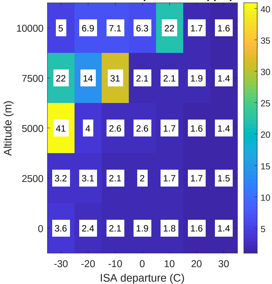
InvGPR PI + FF: Speed RMSE (rpm)
