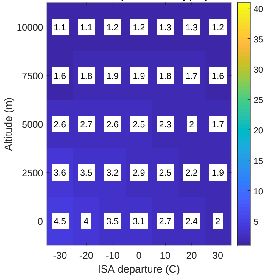
Base PI: Speed RMSE (rpm)
