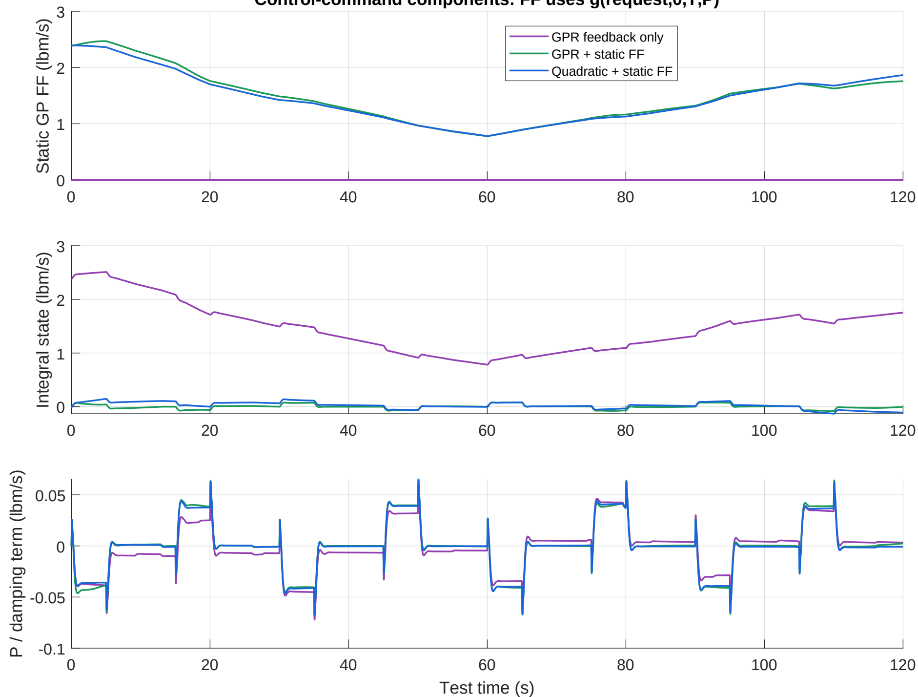
Control-command components: FF uses g(\text{request}, 0, T, P)
