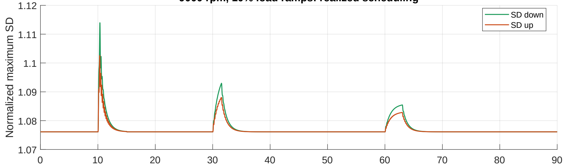
9000 rpm, 10% load ramps: realized scheduling
