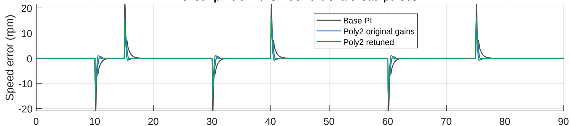
9250 rpm / 0 m / ISA 0 / 10% shaft-load pulses
