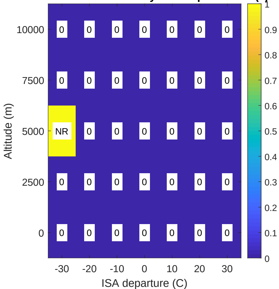
InvGPR PI + FF: Recovery to 1% speed band (s)
