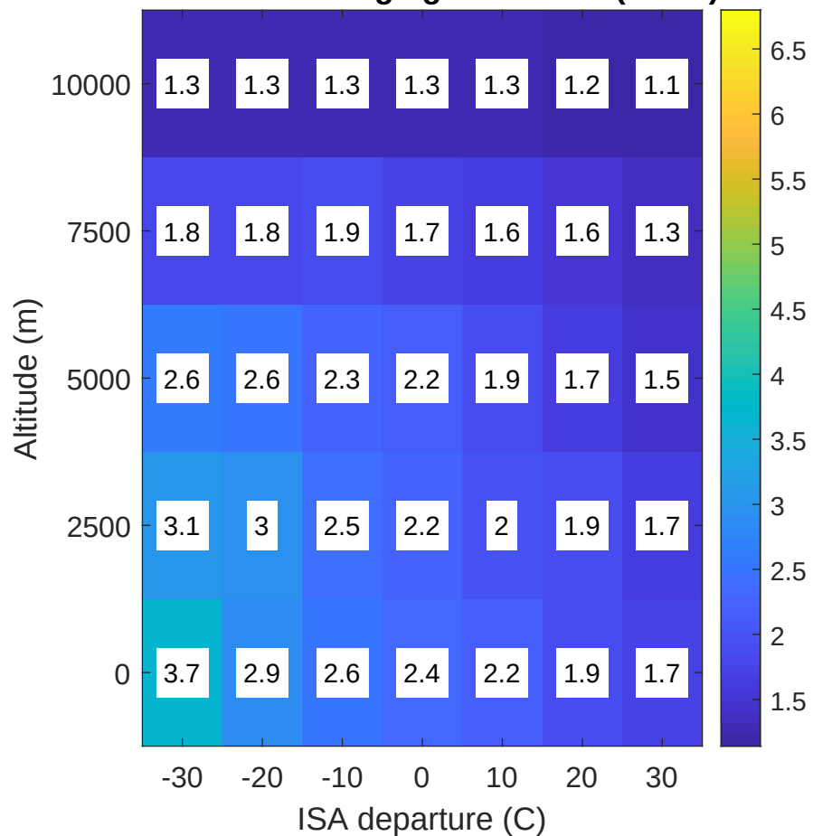
Base PI: Fuel ringing excess TV (lbm/s)
