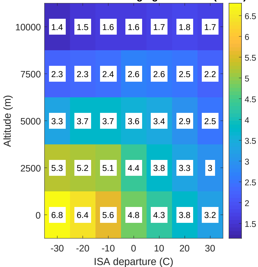
InvGPR PI + FF: Fuel ringing excess TV (lbm/s)
