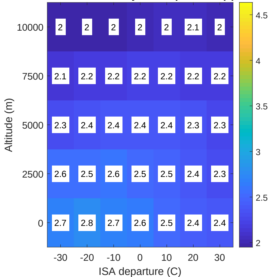
Base PI: Recovery to 0.1 rpm band (s)
