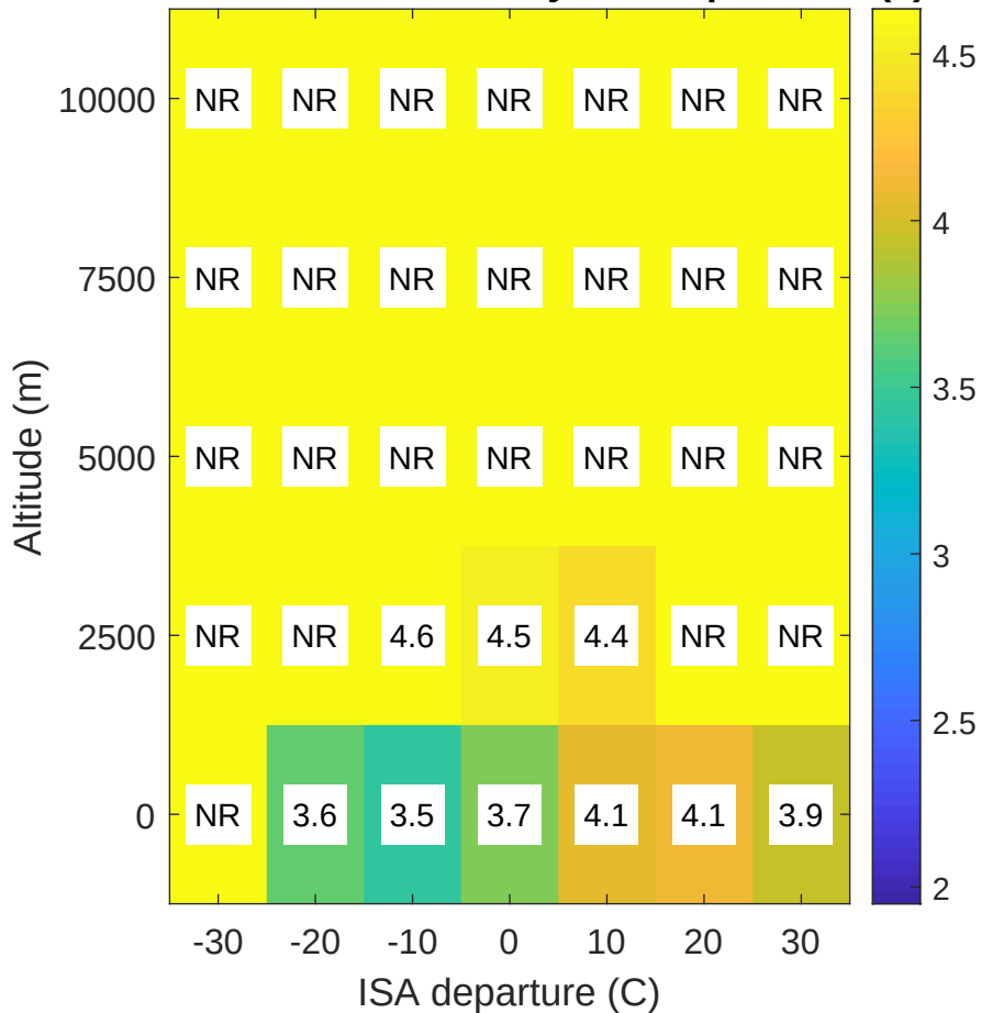
InvGPR PI + FF: Recovery to 0.1 rpm band (s)
