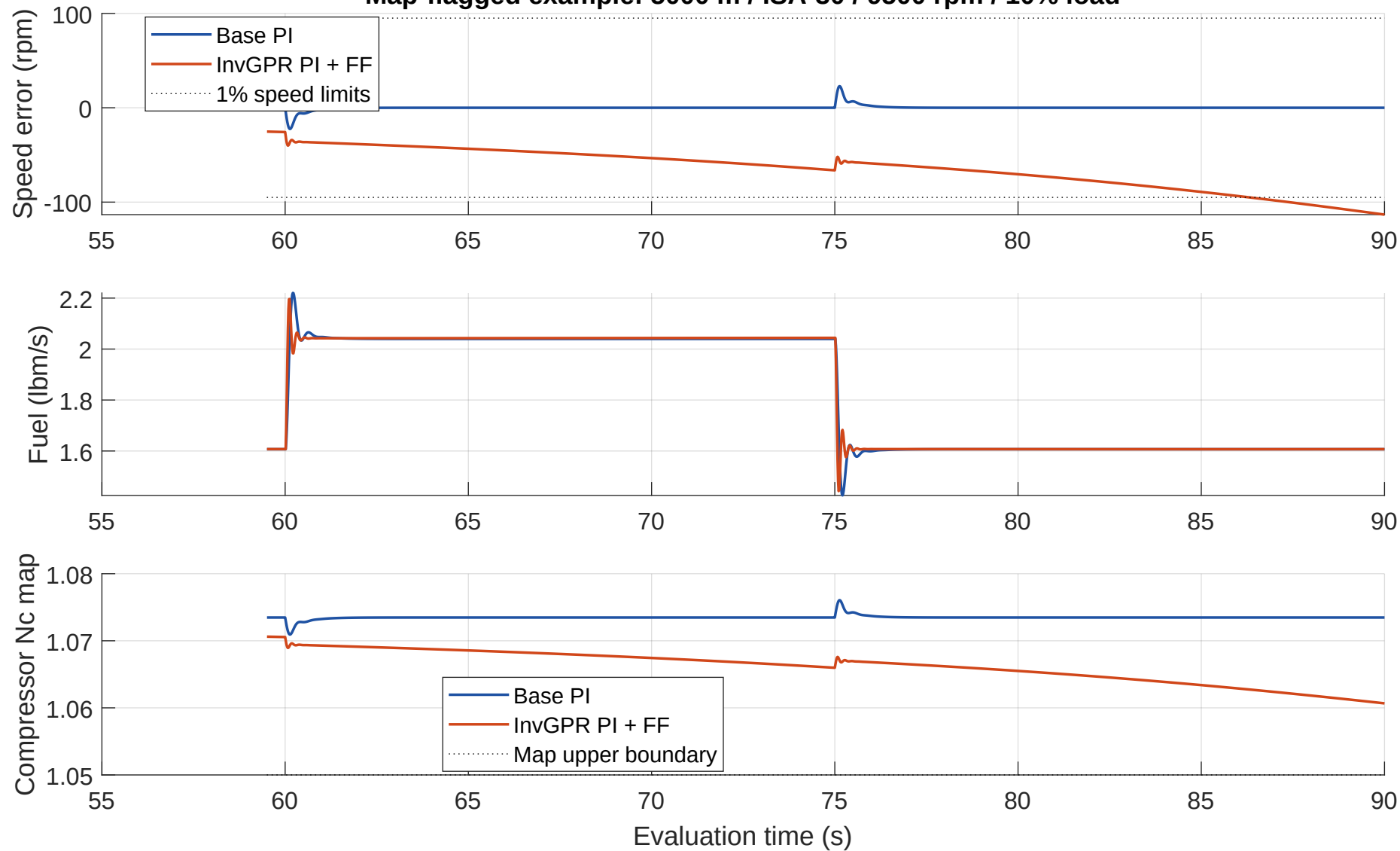
Map-flagged example: 5000 m / ISA-30 / 9500 rpm / 10% load
