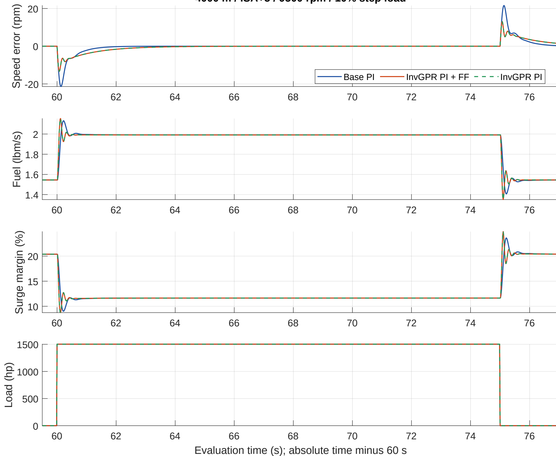
4000 m / ISA+5 / 9500 rpm / 10% step load
