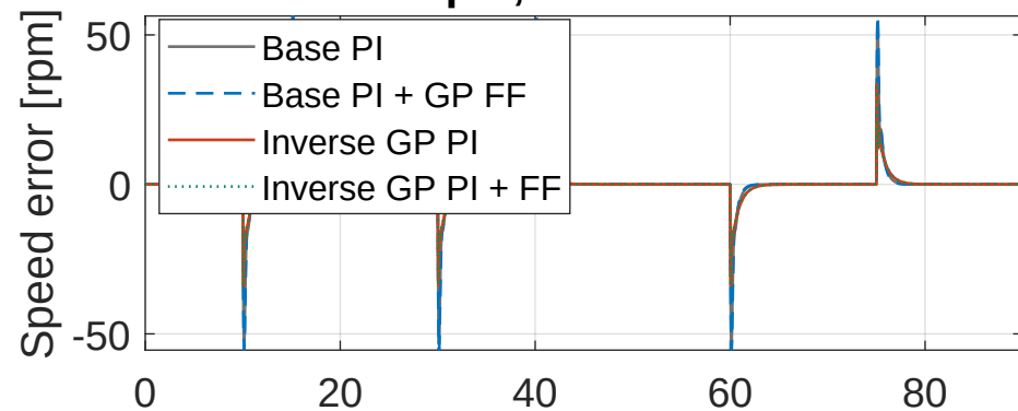
9500 rpm, 30% shaft load
