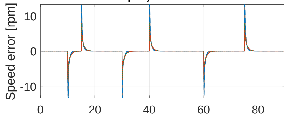
9500 rpm, 5% shaft load
