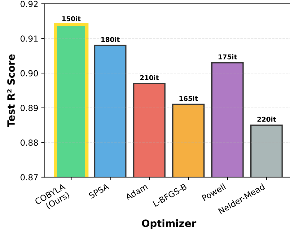
F. Optimizer Comparison
