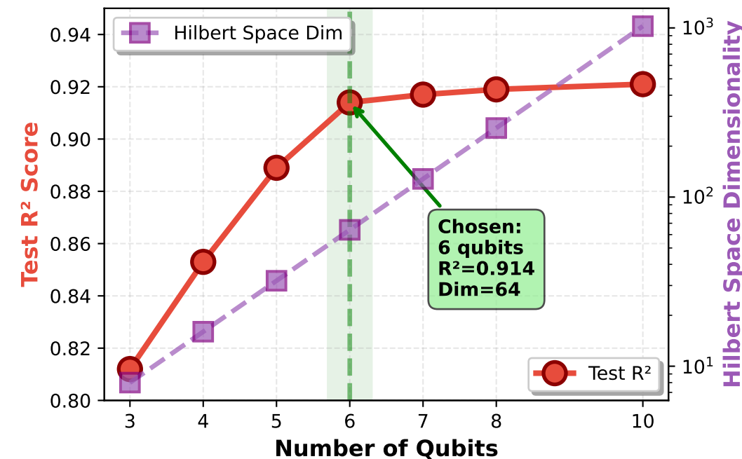
D. Effect of Qubit Count
