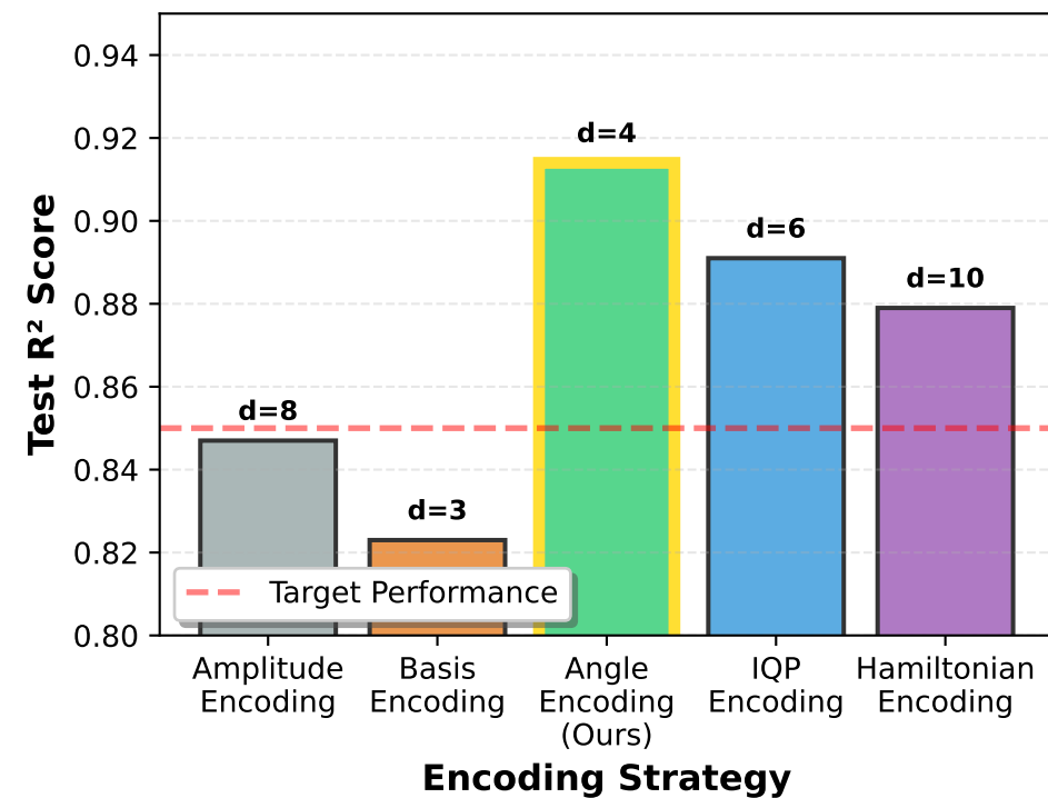
E. Feature Encoding Strategy Comparison
