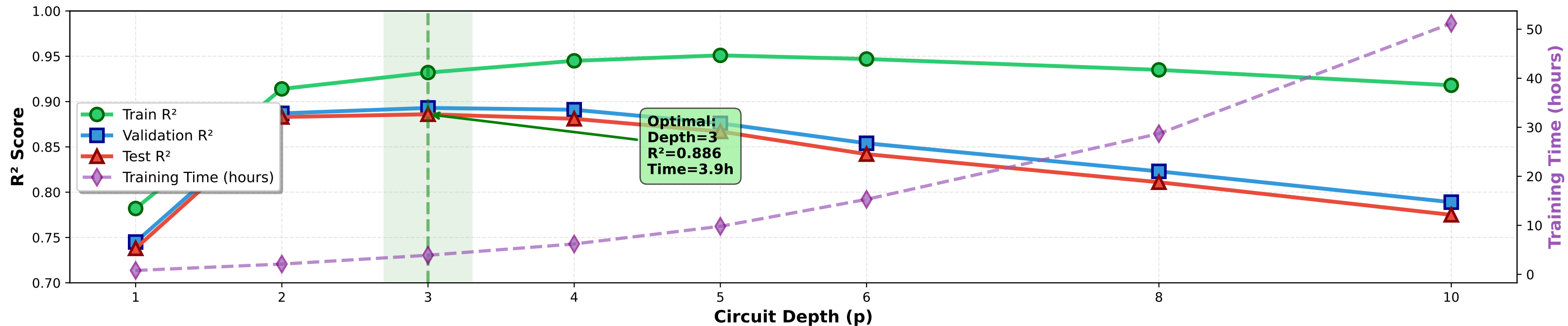
A. Effect of Circuit Depth on Performance and Training Time
