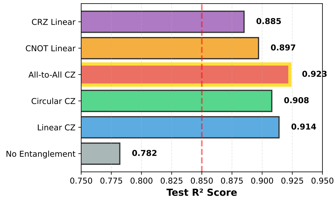
B. Entanglement Pattern Comparison
