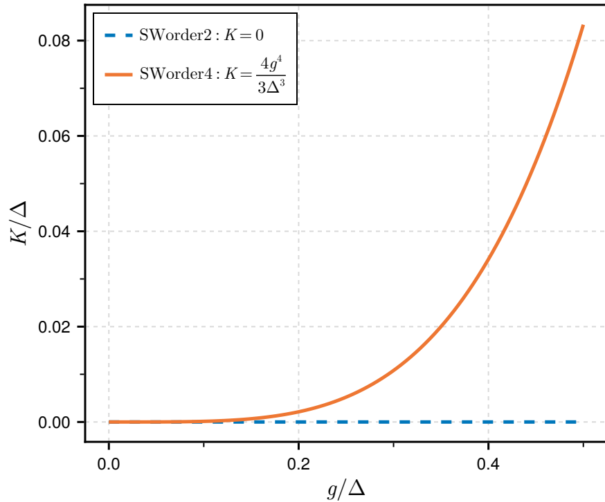
(b) Kerrnonlinearity K(a^\dagger a)^2
