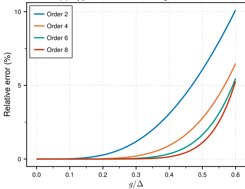
(c) Approximation error in ground state
