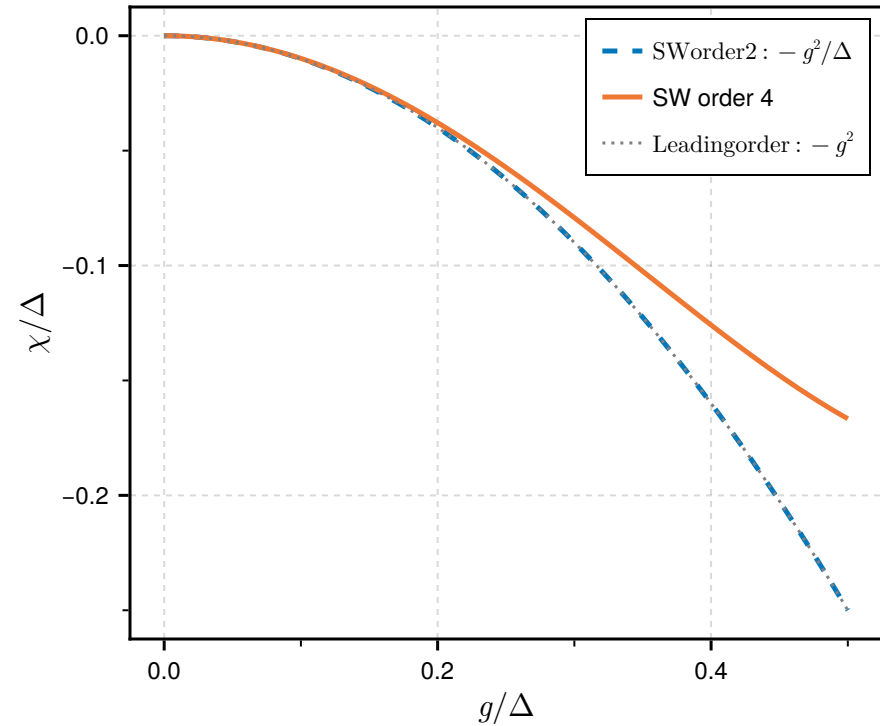
(a) Dispersive shift
