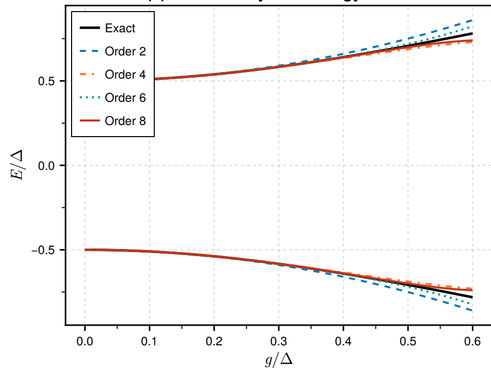
(a) Two-level system energy levels
