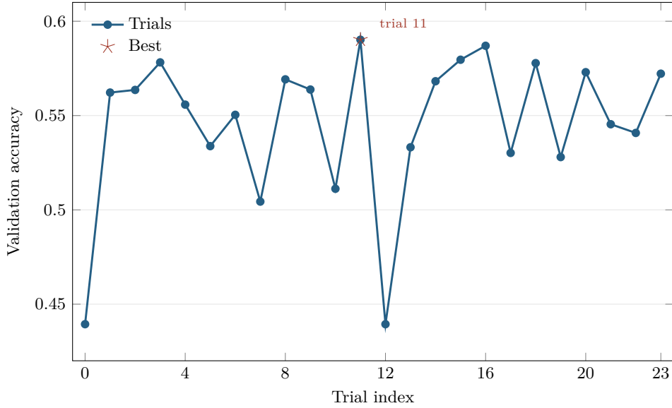
Figure 3: Validation accuracy across the 24 fixed CIFAR-100 sweep trials. The highlighted star marks trial 11, which reached 0.5902 under the 50-epoch sweep budget and was selected for full retraining.
