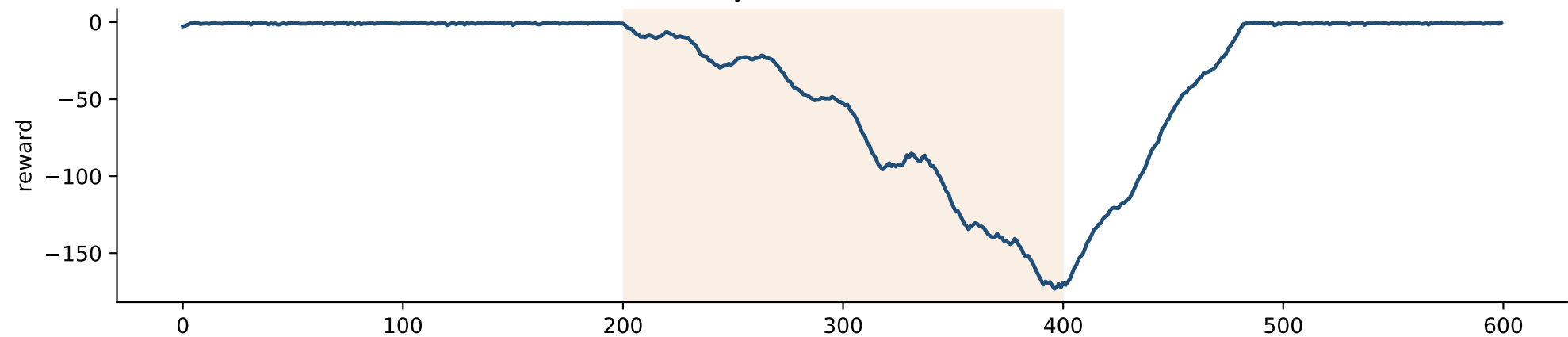
Inventory Control / DQN / seed 11
