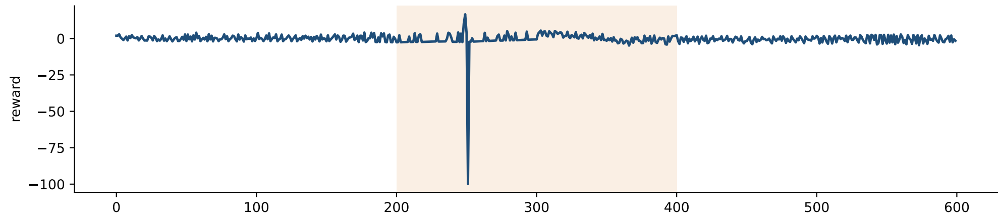
LunarLander Control / DQN / seed 11
