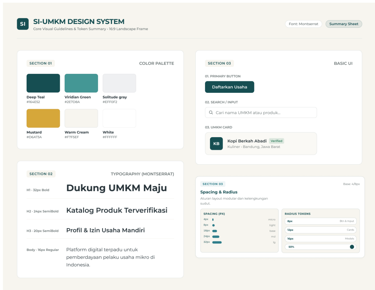
Fig. 3. Design System Antarmuka SI-UMKM Jabar.
