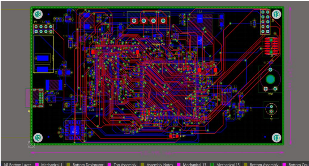
Figure 8 — Altium PCB view with top/bottom routing and internal planes visible.
