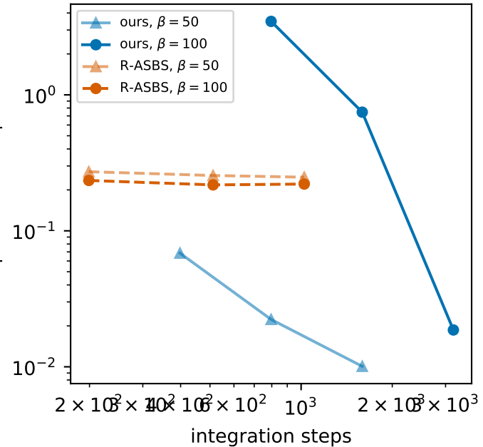
D: error vs steps at \beta = 50, 100 (ours converges, theirs floors)
