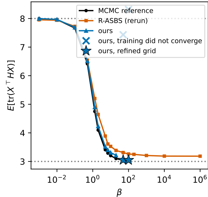
A: expected energy vs \beta (dotted: exact limits 8 and 3)
