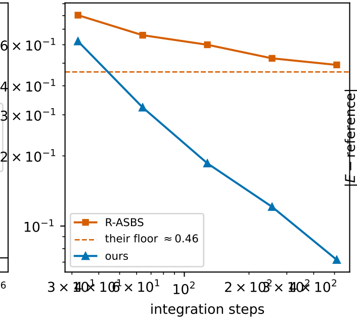
C: error vs steps at \beta = 2
