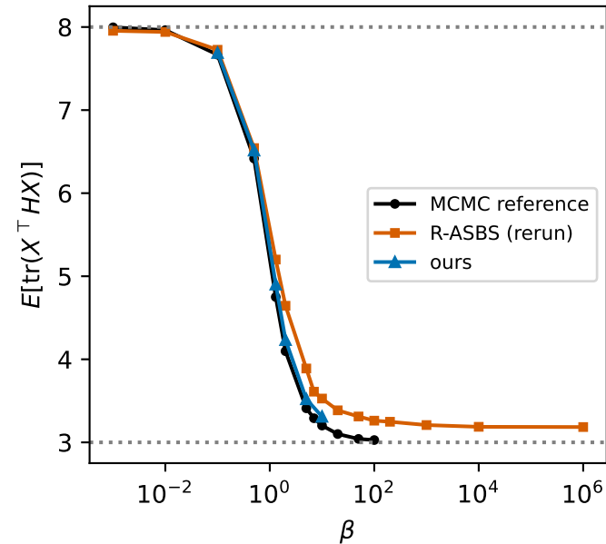
A: expected energy vs \beta (dotted: exact limits 8 and 3)
