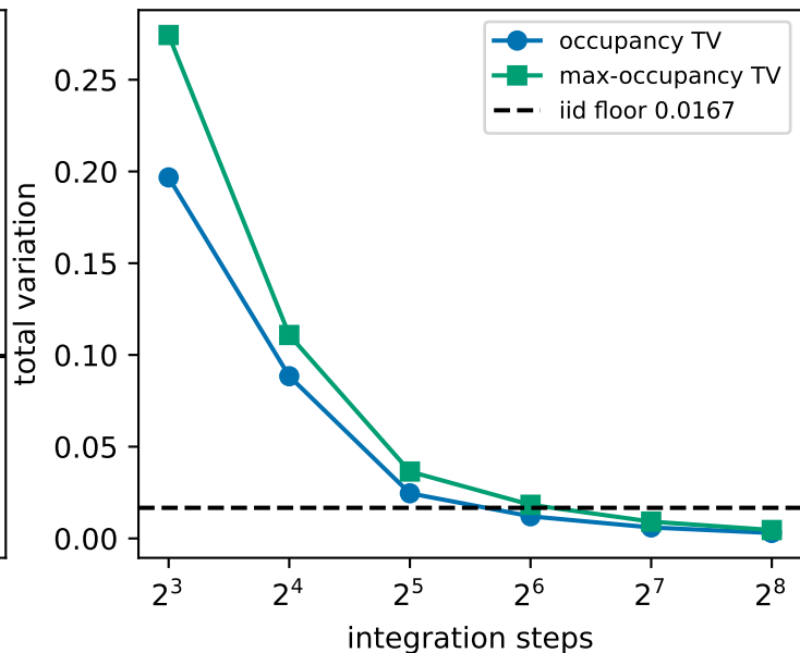
B: occupation model violations = 0
