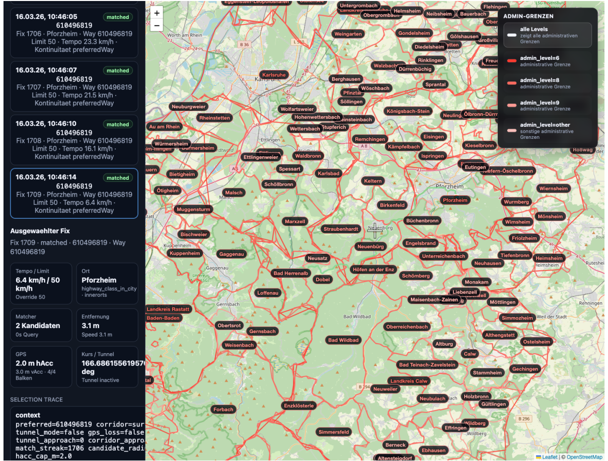
Figure 3: Inspector web app used for replay analysis and per-fix matcher debugging. The view combines fix summaries, selection traces, candidate details, and the linked map context.
