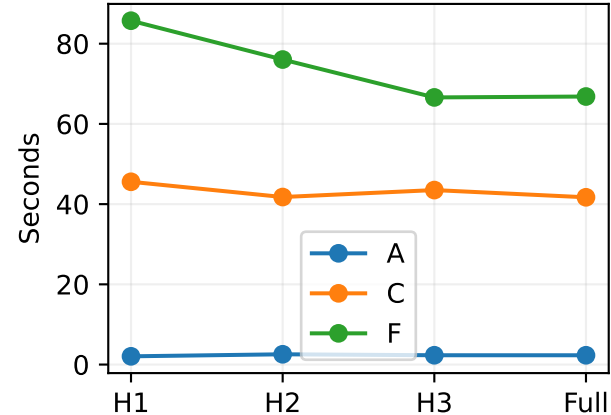
Median latency: H=4, N=2
