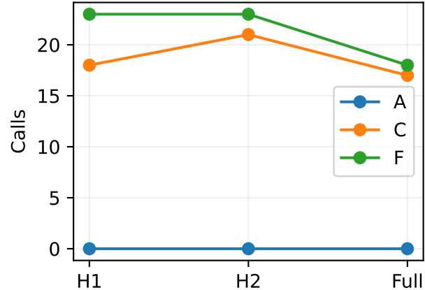
Tool calls/query: H=3, N=1
