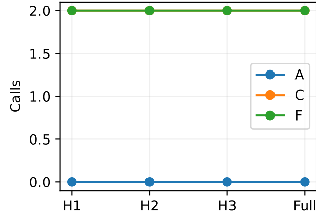
Agent calls/query: H=4, N=2
