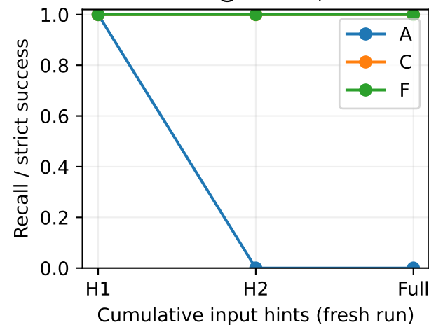
Video R@1: H=4, N=2
