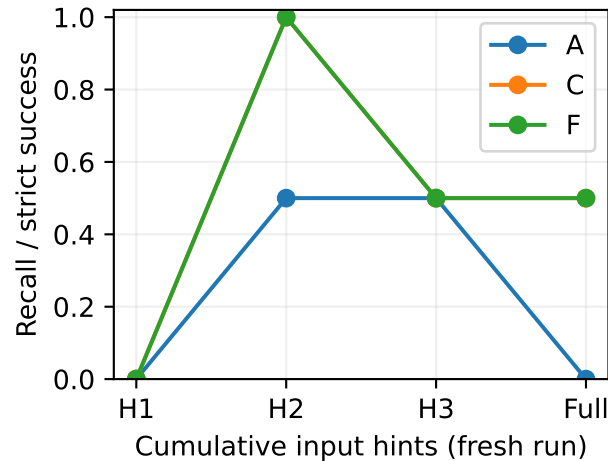
Strict R@1: H=4, N=2
