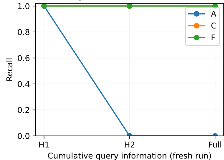
Group strict R@1: 4 hints, N=2
