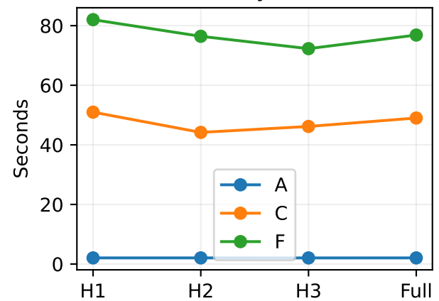
Median latency: H=4, N=20
