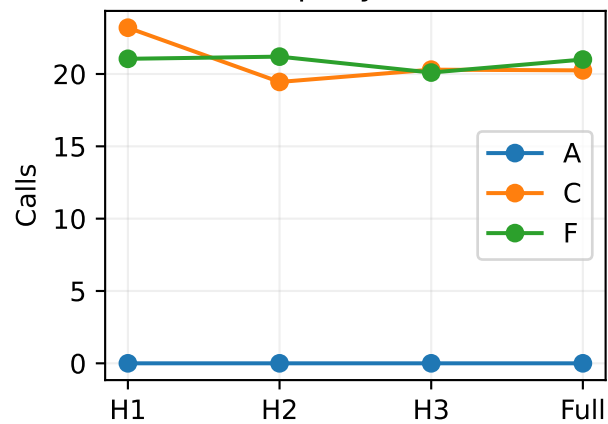
Tool calls/query: H=4, N=20
