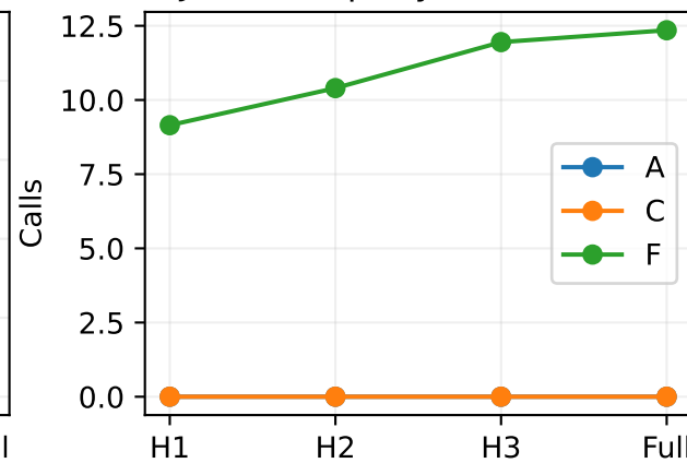
Jev calls/query: H=4, N=20
