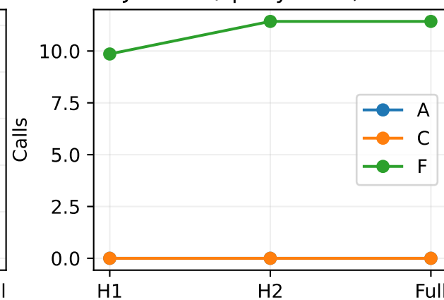
Jev calls/query: H=3, N=7
