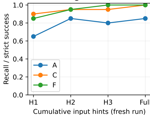
Video R@5: H=4, N=20
