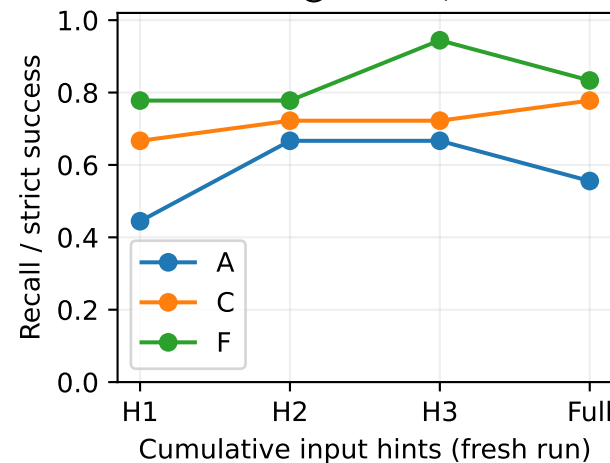
Video R@1: H=4, N=18
