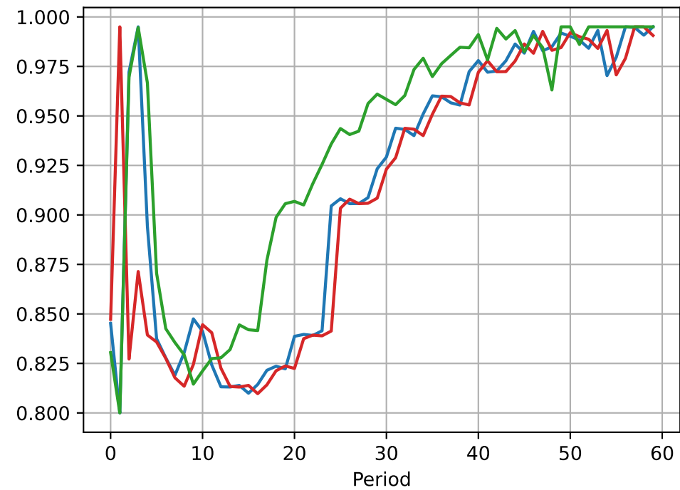
Q (bond price)
