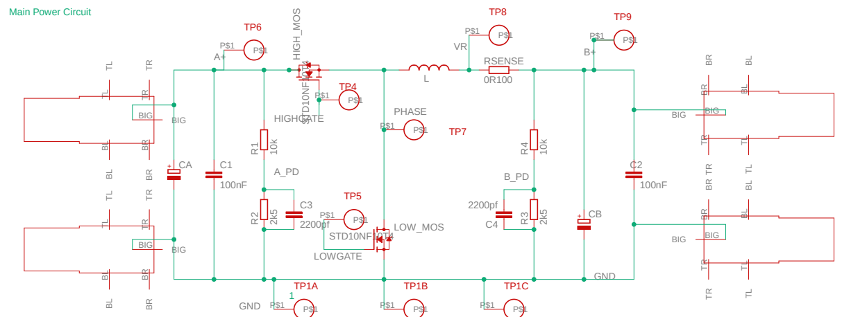
Main Power Circuit
