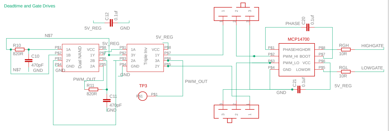
Deadtime and Gate Drives
