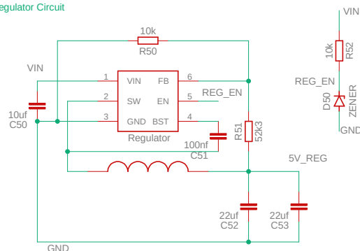
5V Regulator Circuit
