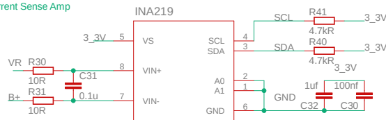
Current Sense Amp
