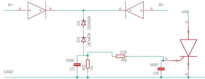
Overvoltage Protection
