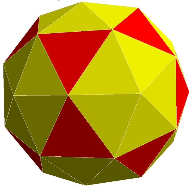
T=4 Pentakis Icosidodecahedron
