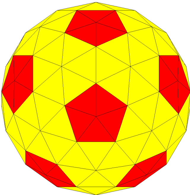
T=9 Conway K6k5tI
