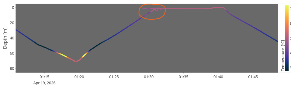
Figure 2: Issue description B (table 2) displayed in temperature data from SEA067 M86. Instance of incorrect timestamps is circled in orange where surface data on following dive is displayed before late dive data. Data displayed and downloaded from VOTO Glider Dashboard [2].
