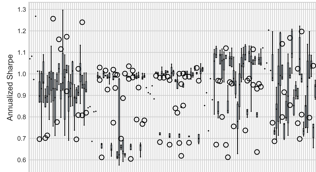
Seed Stability: Annualized Sharpe
