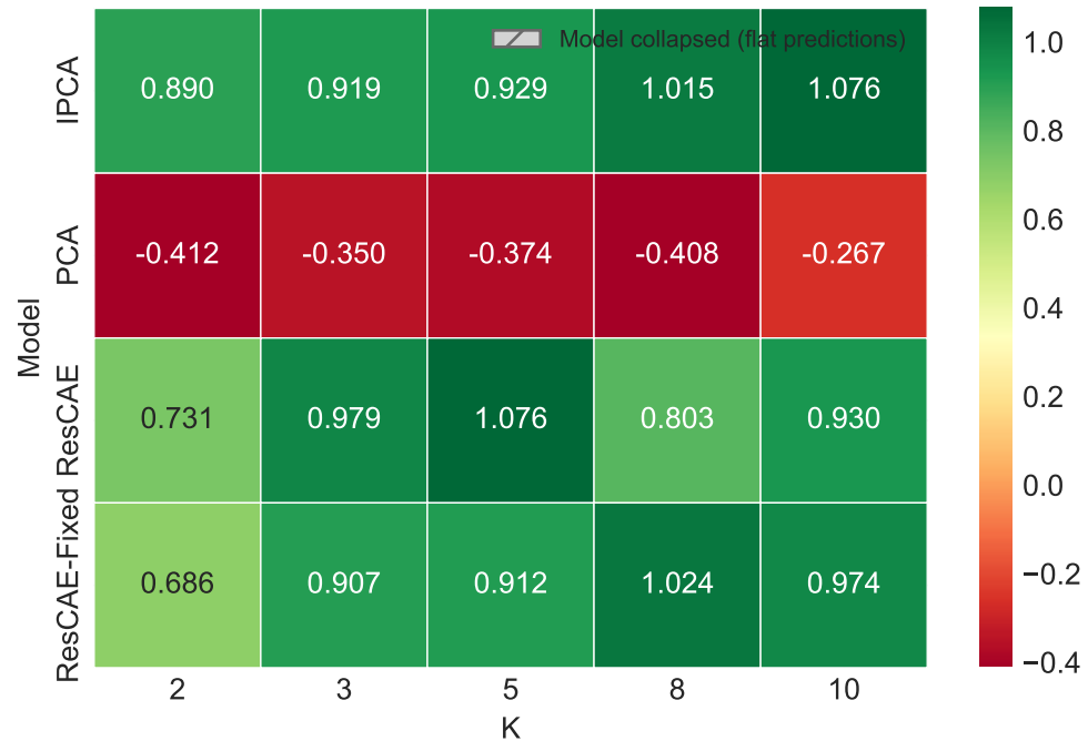
Annualized Sharpe (test set)
