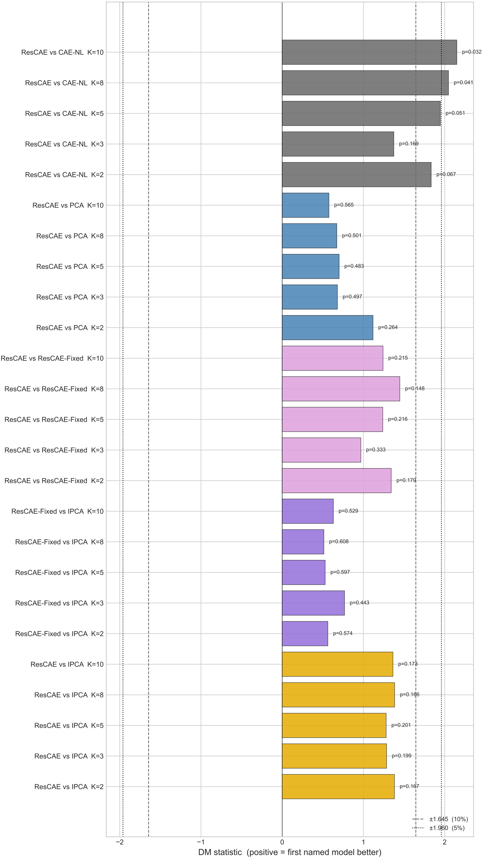
Diebold-Mariano Tests: Does the Nonlinear Residual Add Value?
