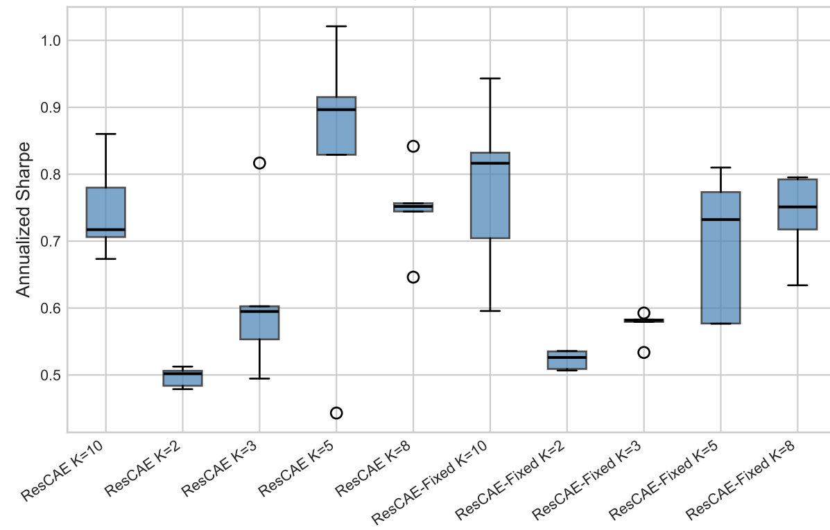
Seed Stability: Annualized Sharpe
