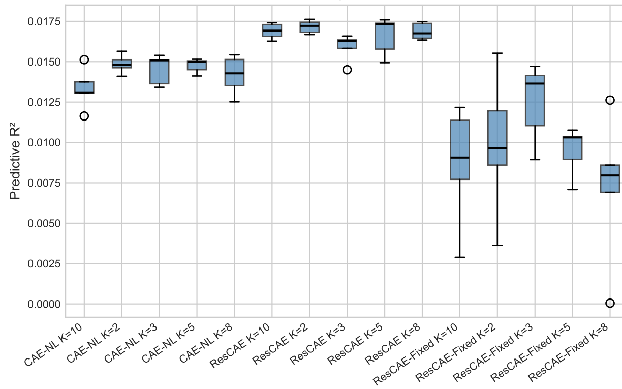
Seed Stability: Predictive R 2
