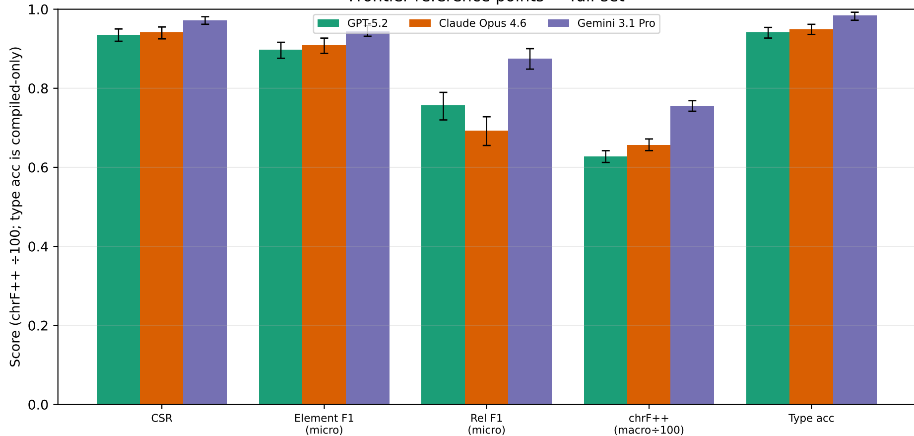
Frontier reference points — full-set
