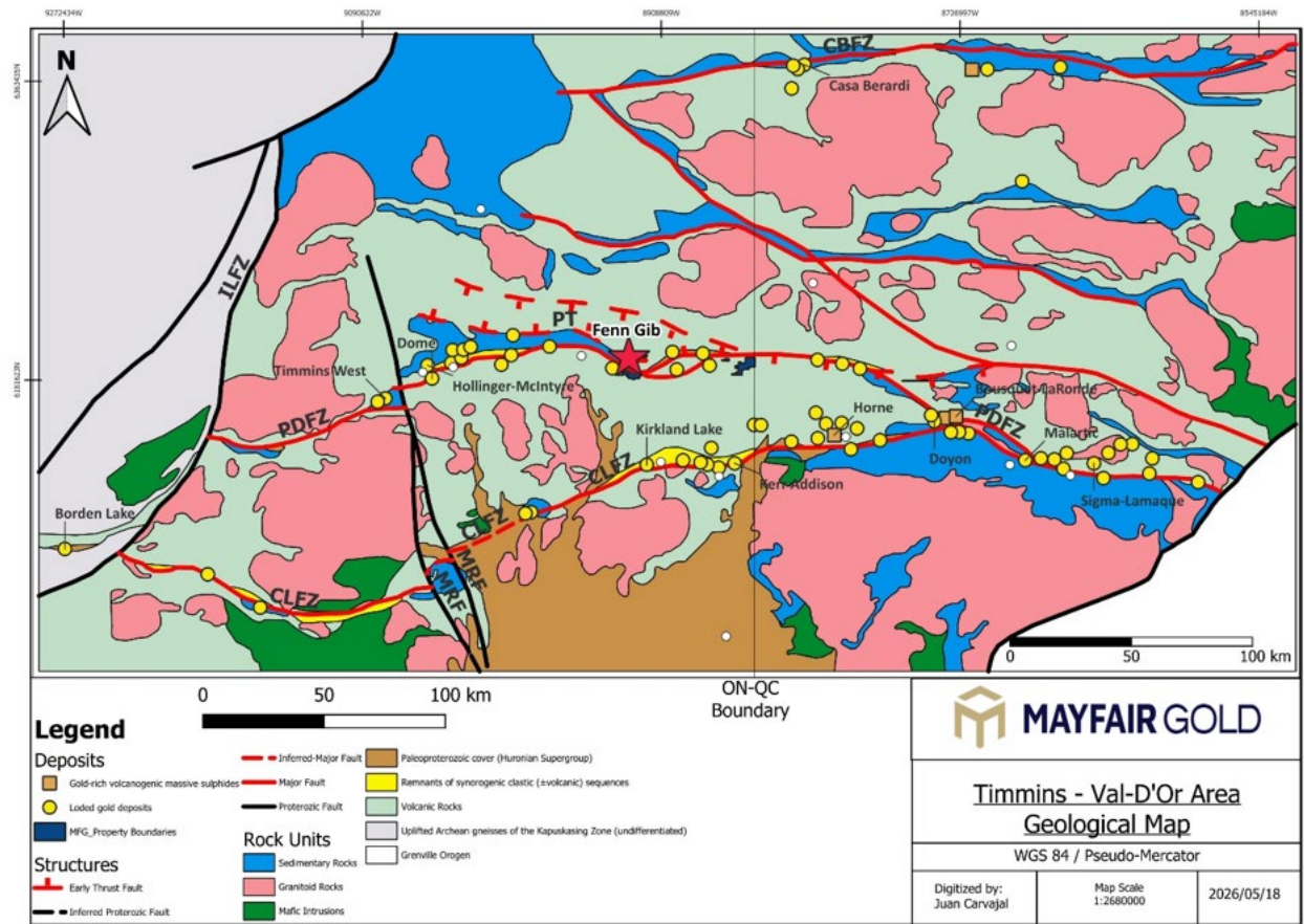
Figure 1: Simplified geological map of the central and southern Abitibi greenstone belt, highlighting major faults and the distribution of gold deposits (modified after Poulsen et al., 2000, and Dubé and Mercier-Langevin, 2015).
