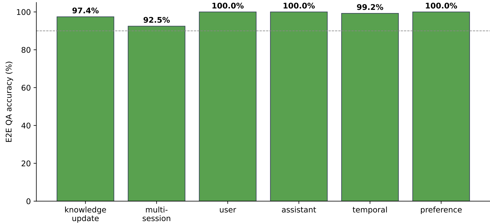
Figure 4 — LongMemEval-S E2E QA by type (paper profile; 487/500 = 97.4%)
