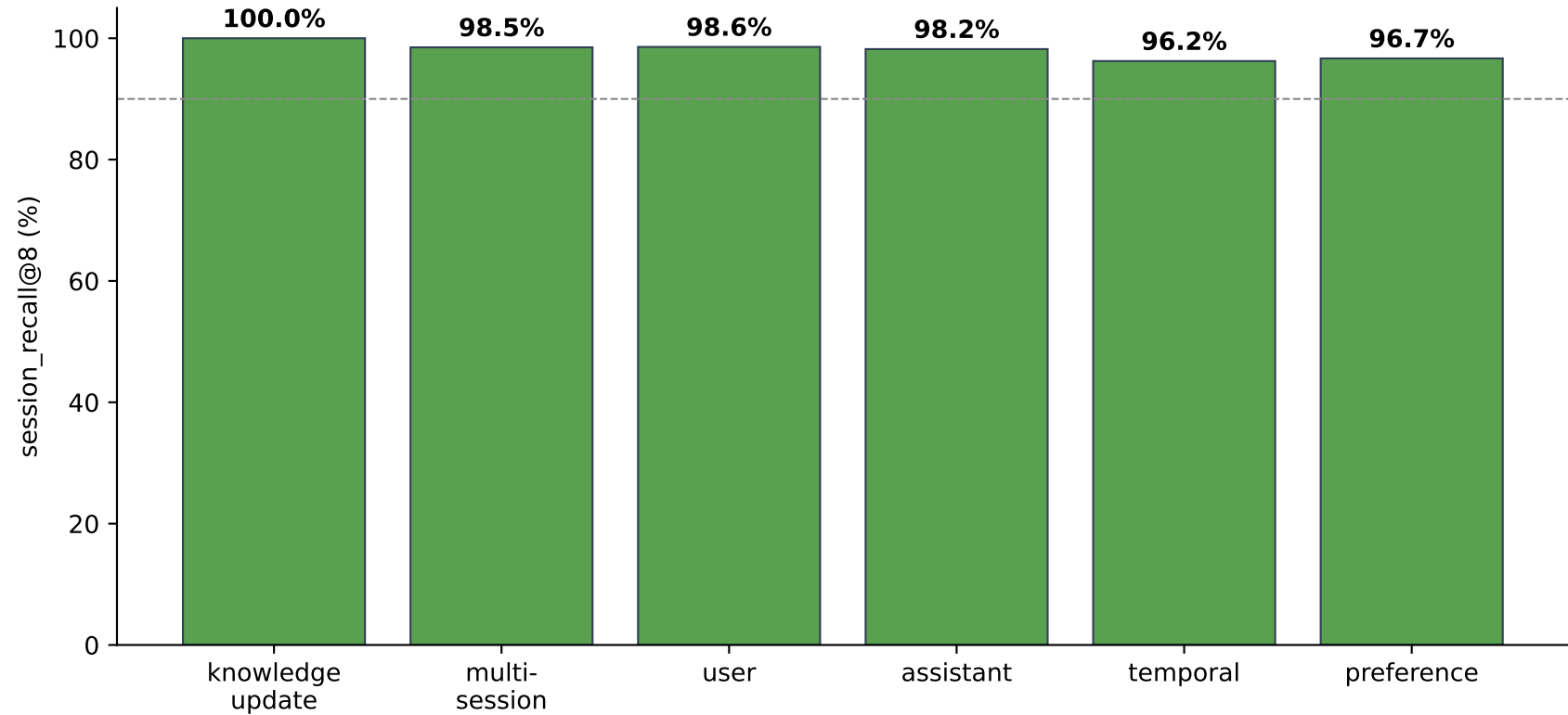
Figure 3 — LongMemEval-S by question type (490/500 overall = 98.0%)
